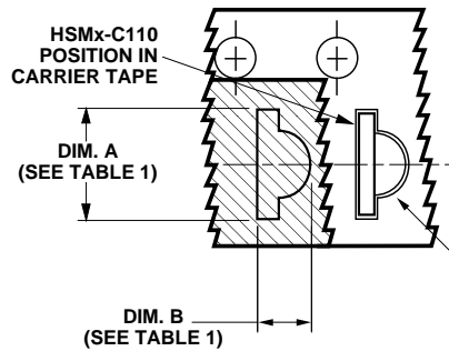
Figure 14. Tape dimensions.
