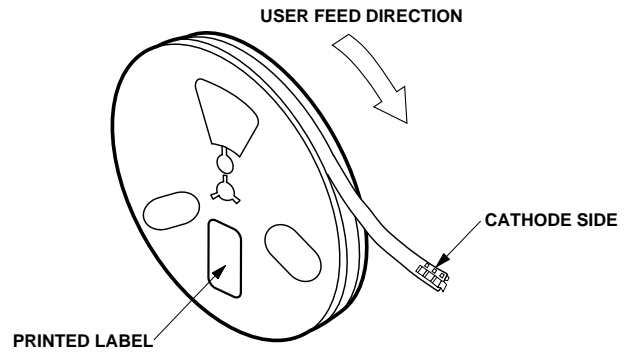
Figure 12. Reeling orientation.
