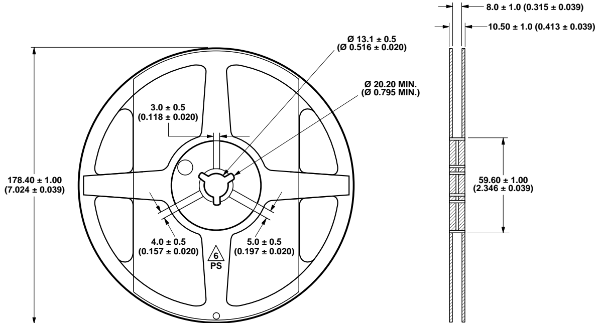
Figure 13. Reel dimensions.
